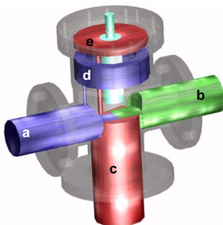
Gas Flow through POM Valve
